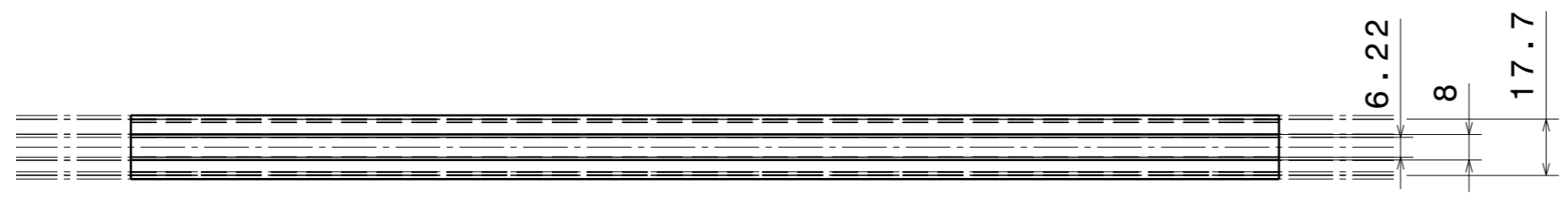
Front view
